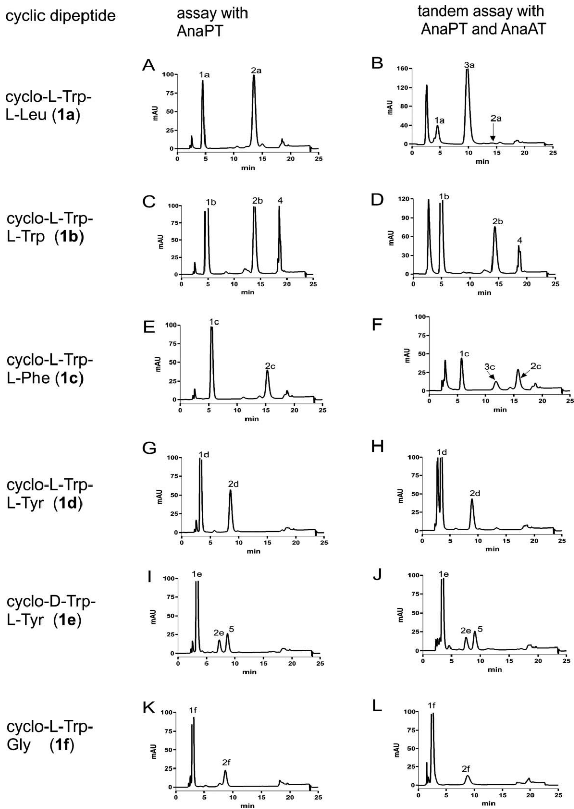
Fig. 2 HPLC chromatograms of incubation mixtures of six tryptophan-containing cyclic dipeptides with recombinant AnaPT or AnaPT and AnaAT. Detection was carried out with a photo diode array detector and illustrated for absorption at 254 nm.
