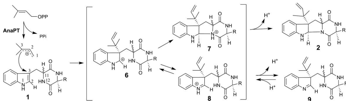
Scheme 2 Possible mechanism of AnaPT reaction.
