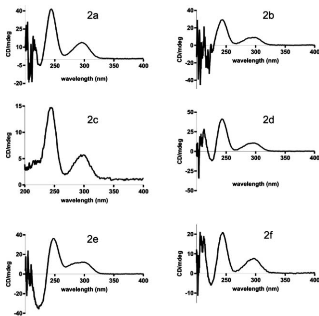
Fig. 3 CD spectra of C3-prenylated pyrrolo[2,3- b ]indoles.
