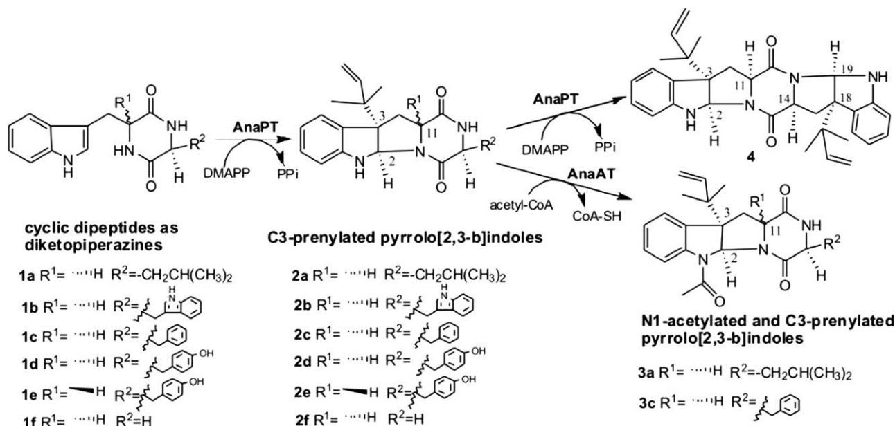
Scheme 1 Chemoenzymatic synthesis of C3-prenylated pyrrolo[2,3-b]indoles by recombinant enzymes.
