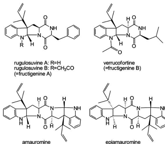
Fig. 1 Examples of C3-prenylated pyrrolo[2,3-b]indoles.
